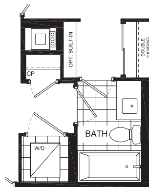
OPTIONAL PRIVACY ENSUITE (AVAILABLE AT DESIGN CENTRE)
