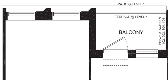
UNIT PART PLAN @ 519, 619, 719
