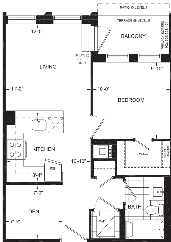
UNIT PART PLAN @ 519, 619, 719
